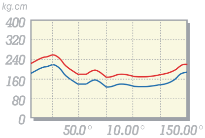
Shown curves refer to PDC200W
